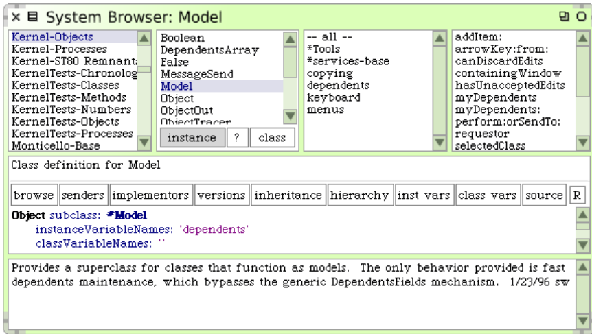
Figure 6.2: System Browser with the class Model selected
